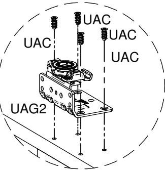
DETAIL 1
