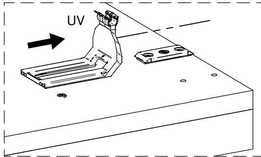
DETAIL 1
