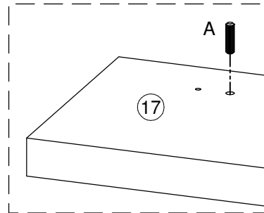
DETAIL 1
