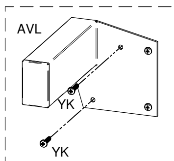
DETAIL 1
