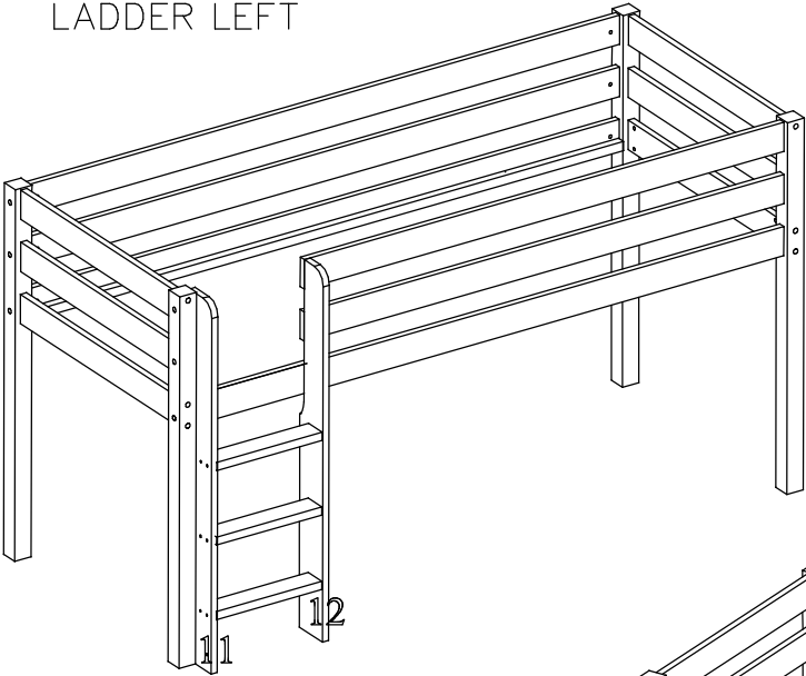
LADDER LEFT
