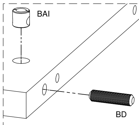
DETAIL 1
