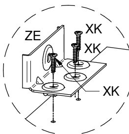
DETAIL 3
