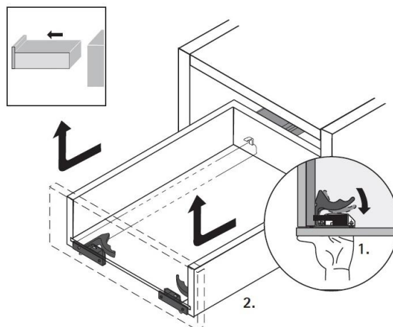
Remove drawer
