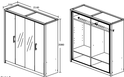
ELIAS MODEL : WR 80185-2M-S5V-P ITEM : KLEERKAST-ARMOIRE 4 D/P / 4 DOORS WARDROBE WITH 2 MIRRORS PRODUCT SIZE : L 214 X D 55 X H 208cm
