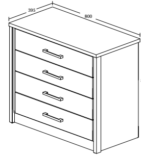
ELIAS MODEL : COD 5963-S5V-P ITEM : COMMODE 4 S/T/ 4 DRAWERS CHEST PRODUCT SIZE : L 80 X D 39.5 X H 83cm
