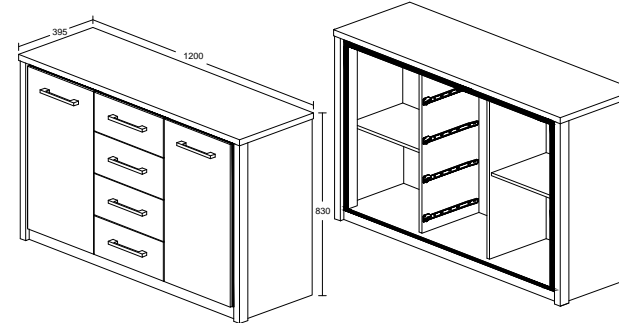
ELIAS MODEL : DTC 357-S5V-P ITEM : COMMODE 2 D/P - 4 S/T/ CHEST PRODUCT SIZE : L 120 X D 39.5 X H 83cm
