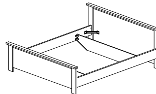
ELINE MODEL : BED 70-6379C-S5V ITEM : BED-LIT 160 L 209 X D 178 X H 95cm M/S: L160 X 200 cm
