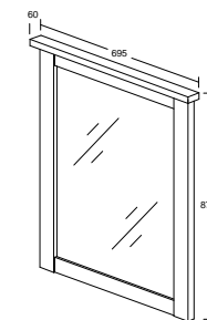
ELLA MODEL : HM 2502-S5V ITEM : SPIEGEL MIROIR / HANGING MIRROR L 69.5 X D 6 X H 87 cm
