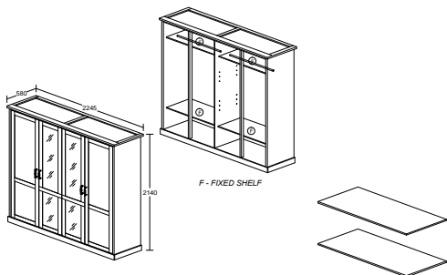
ELLA MODEL : WR 80098-2M-S5V ITEM : KLEERKAST / ARMOIRE 4D/P / 4 DOORS WARDROBE WITH 2 MIRRORS L 224.5 X D 58 X H 214 cm
