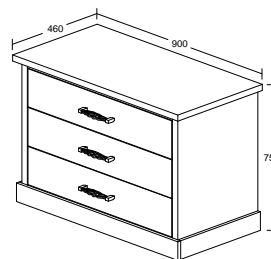
ELLA MODEL : COD 5921-S5V ITEM : COMMODE 3 LT / CHEST OF 3 DRAWERS L 90 X D 46 X H 75.5 cm
