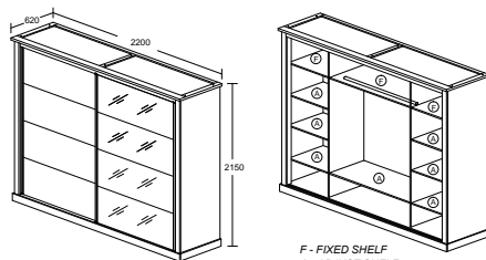
F - FIXED SHELF A - ADJUST SHELF
