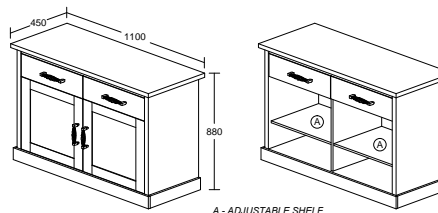
A - ADJUSTABLE SHELF
