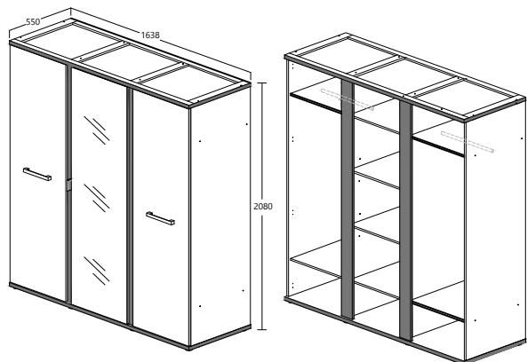
ELLEN MODEL : WR 80208-1M-S5V ITEM : 3 DOORS WARDROBE WITH 1 MIRROR L 163.8 X D 55 X H 208cm
