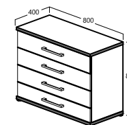
ELLEN MODEL : COD 5971-S5V ITEM : CHEST OF 4 DRAWERS L 80 X D 40 X H 82cm
