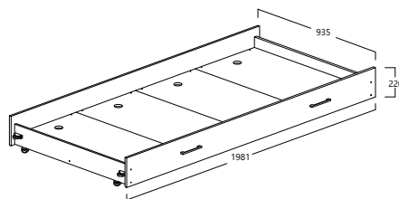
ELLEN MODEL : BED 59-S5V ITEM : BED DRAWER L 198.1 X D 93.5 X H 22cm
