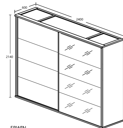
ERWIN MODEL : WR 80229-4M-FO-S5V ITEM : KLEERKAST / ARMOIRE 2D / P/ 2 DOORS WARDROBE WITH 4 MIRRORS L 240 X D 60 X H 214cm
