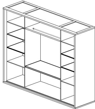
ERWIN MODEL : WR 80216-4M-FO-S5V ITEM : KLEERKAST / ARMOIRE 2D / P/ 2 DOORS WARDROBE WITH 4 MIRRORS L 200 X D 60 X H 214cm
