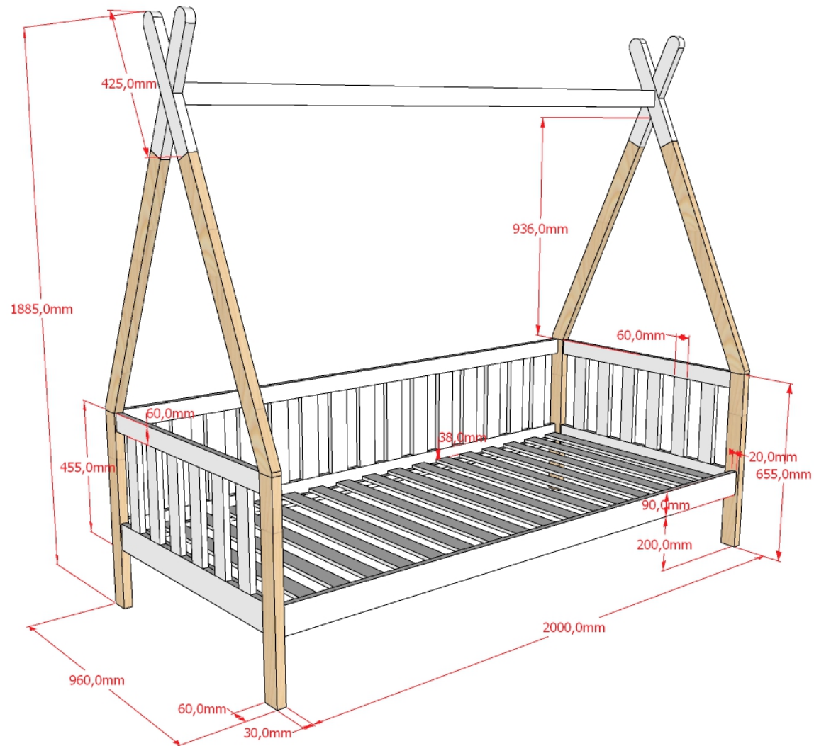
TIPI BED : TIBEHK9014 L:2060mm H:1885mm D:960mm INNERSIZE 900x2000mm 17 slats 60x12mm
