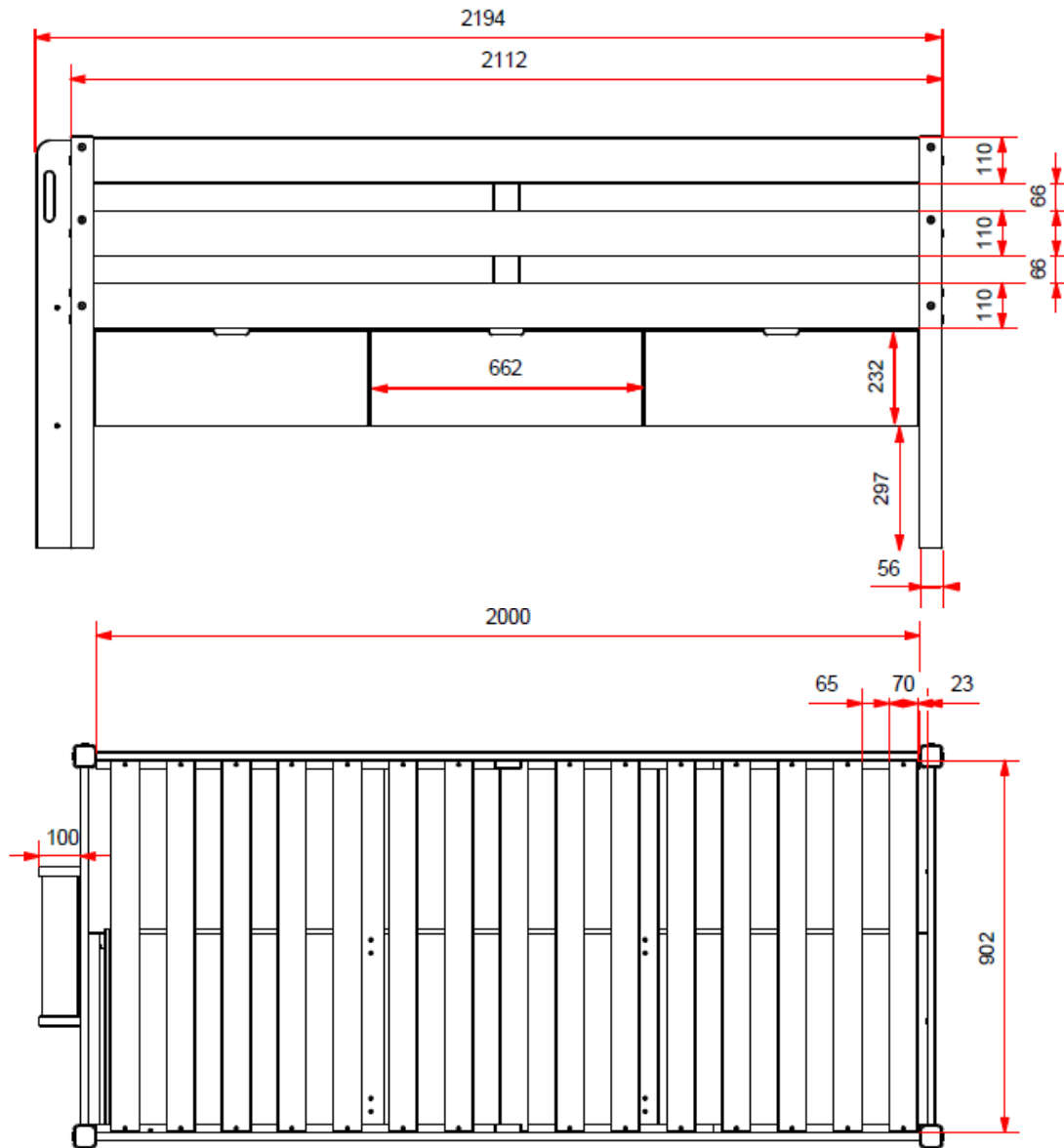
L: 2194mm H: 1000mm D: 978mm INNERSIZE 2000x900mm
