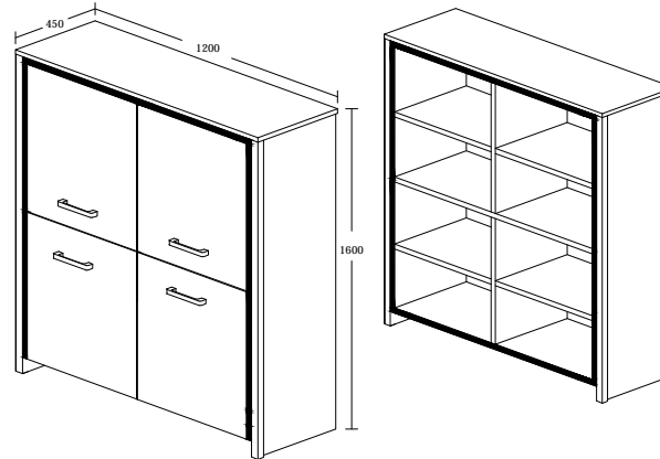
MODEL : MC 5046-S5V-P ITEM : ELIAS BAR 120 / 4 DOORS CABINET COLOR : NEW GREY OAK + BLACK LINE PRODUCT SIZE : L 120 x D 45 x H 160cm
