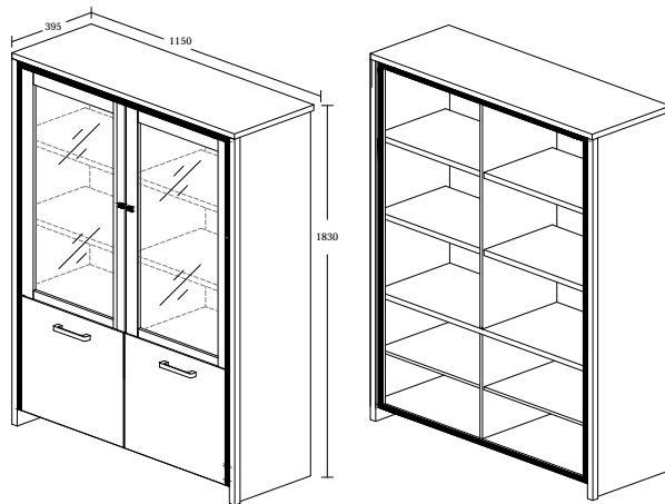
MODEL : BC 70099G-S5V-P ITEM : ELIAS GLASKAST-ARGENTIER / GLASS CABINET COLOR : NEW GREY OAK + BLACK LINE PRODUCT SIZE : L 115 x D 39.5 x H 183cm
