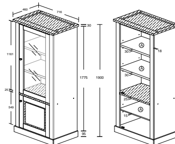
EMMA MODEL : TW 17014-TG-S5V ITEM : TOWER WITH GLASS DOOR L 71.6 X D 46 X H 190 cm
