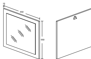
EMILY / EMMA MODEL : 1304-HC-S5V ITEM : SPIEGEL / MIROIR / MIRROR L 55 X D 1.5 X H 55 cm
