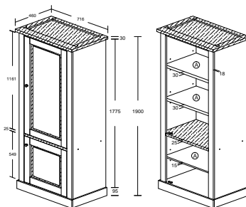
EMMA MODEL : TW 17015-TP-S5V ITEM : TOWER WITH WOODEN DOOR L 71.6 X D 46 X H 190 cm
