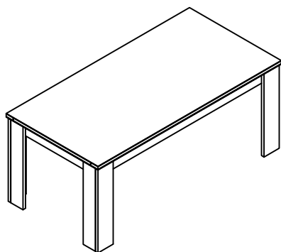
ENZOR MODEL :DN DT 660 103 ITEM :EETTAFEL / TABLE / DINING TABLE 180 L 180 X D 90 X H 75 CM
